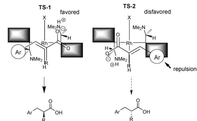
Figure 3. Transition-state models for the asymmetric hydrogenation of \alpha -substituted cinnamic acids catalyzed by the (R_C, R_C, S_{FC}, S_{FC}, S_P, S_P) - 1 -Rh complex.
