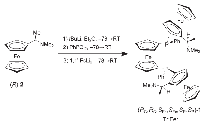
Scheme 1. Preparation of ligand 1 .
